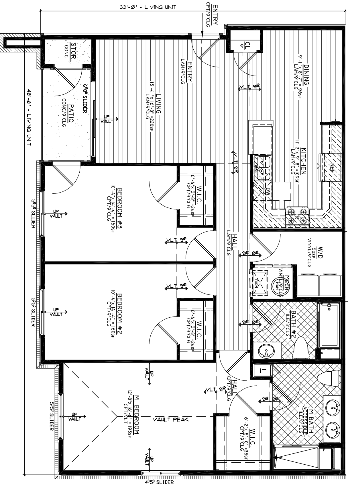
1 MODEL 1555 - UPPER CORNERS GRAPHIC SCALE LIBERTY PLAN (6.21)
