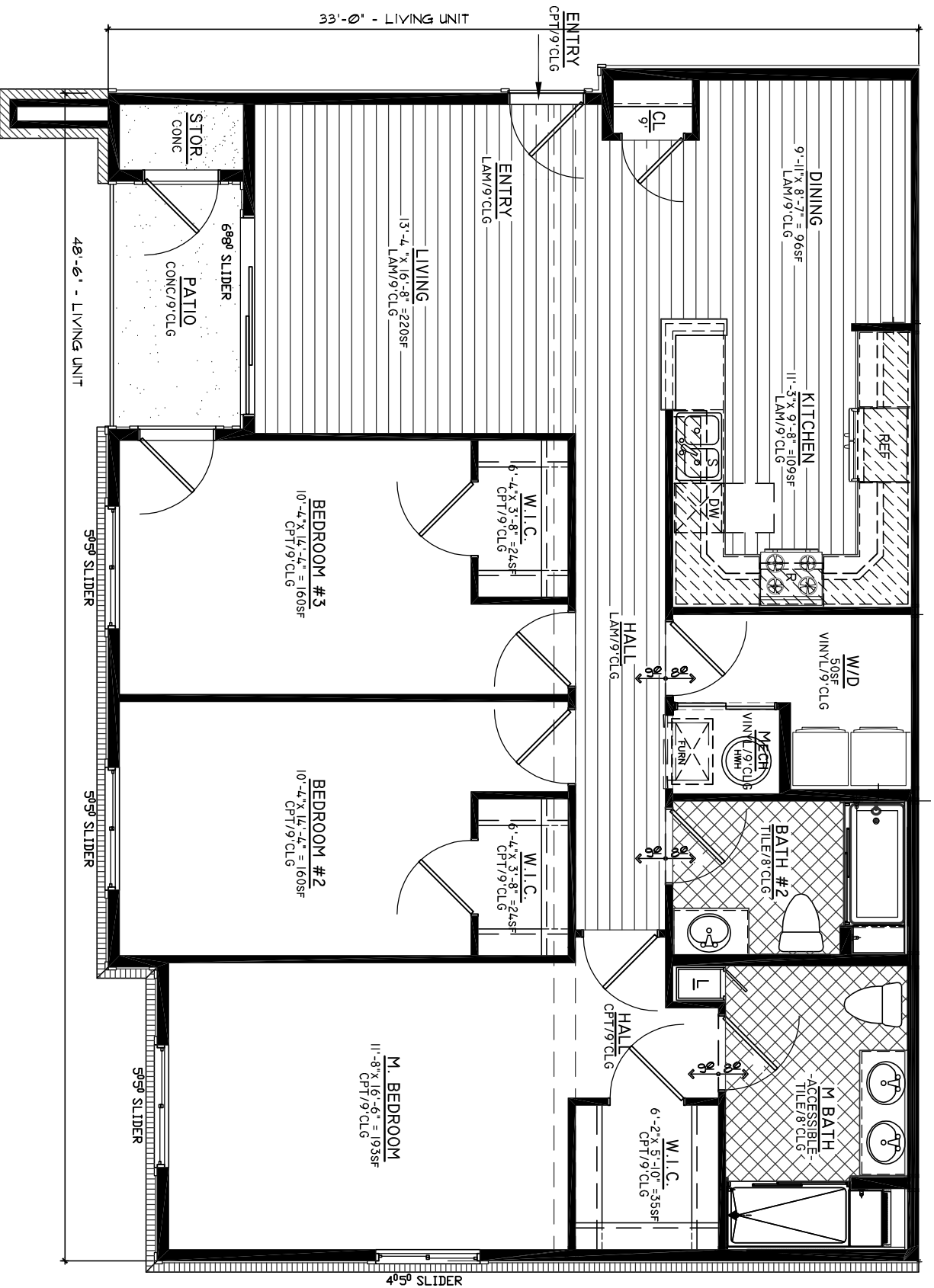
1 MODEL 1555 - 2ND LEVEL GRAPHIC SCALE LIBERTY PLAN (6.21)
