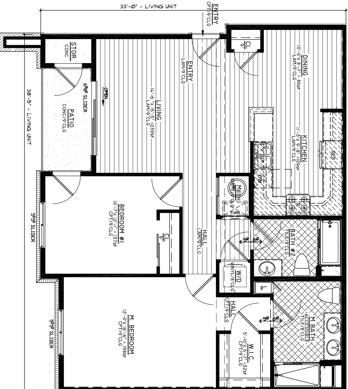
1 MODEL 1255 - 2ND LEVEL INT GRAPHIC SCALE ORLEANS PLAN (6.21)
